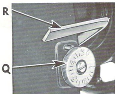
Fig. 28. Regulating Stitch Length
