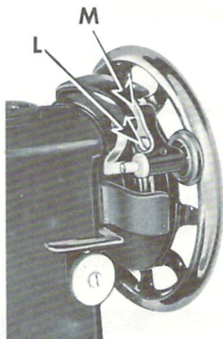
Fig. 16. Adjusting Bobbin Winder
