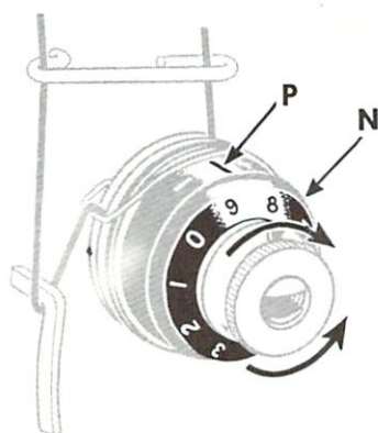
Fig. 25. Regulating Needle Thread Tension
