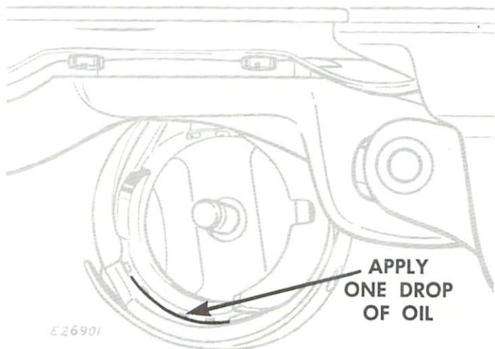
Fig. 7. Oiling Point in Hook Race
