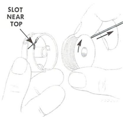
Fig. 17. Placing Bobbin in Bobbin Case
